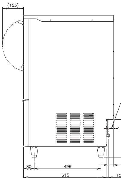
RIGHT SIDE
