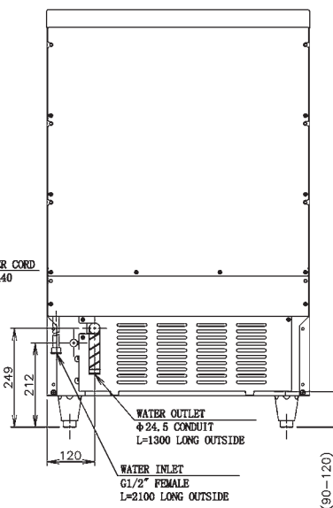
BACK SIDE
